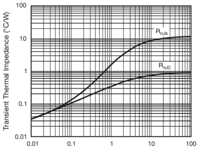
FIGURE 5 Typical Transient Thermal Impedance
